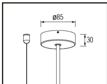
Round canopy
