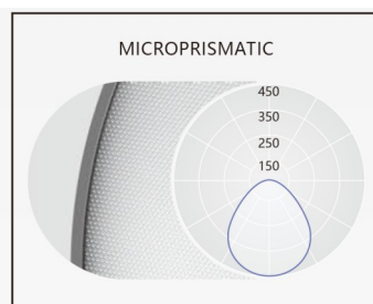
Prismatics diffuser for UGR<19
